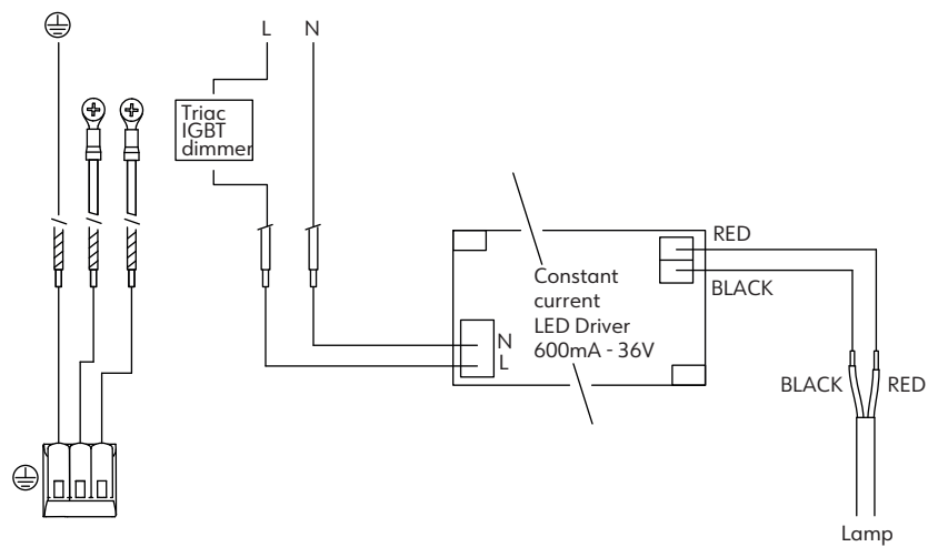
PHASE CUT DIMM wiring diagram
