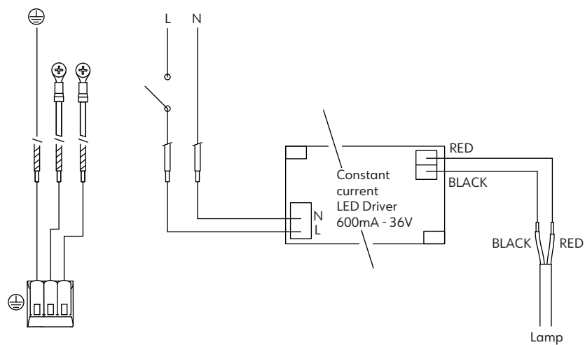
ON-OFF wiring diagram
